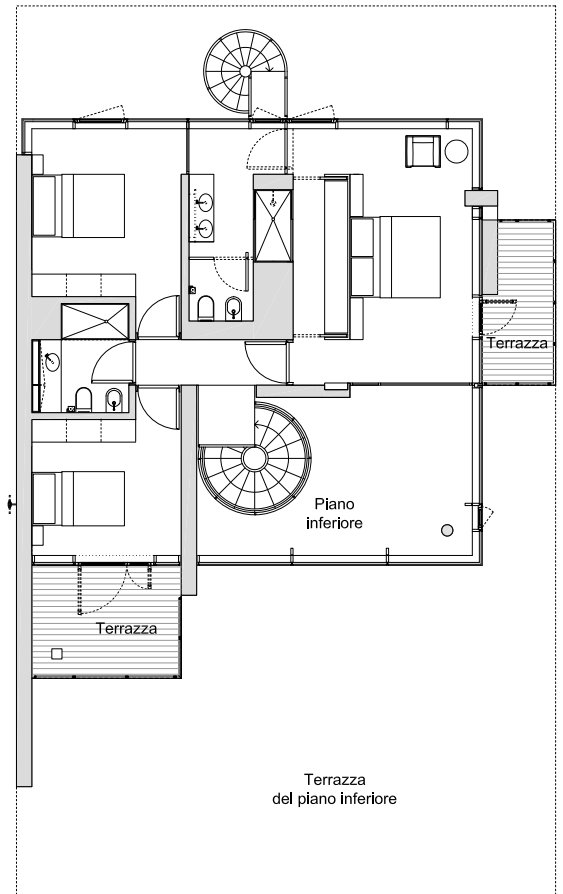
Piano Superiore
